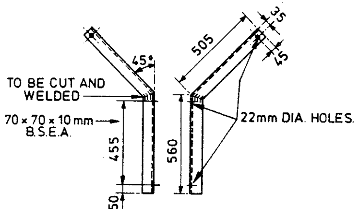
SUPPORTING BRACKETS (TO BE SUPPLIED IN PAIRS)
